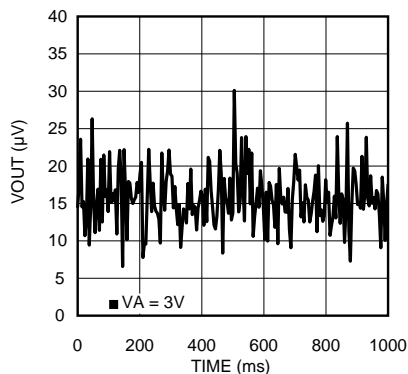
Noise Measurement without Calibration at Gain = 8
