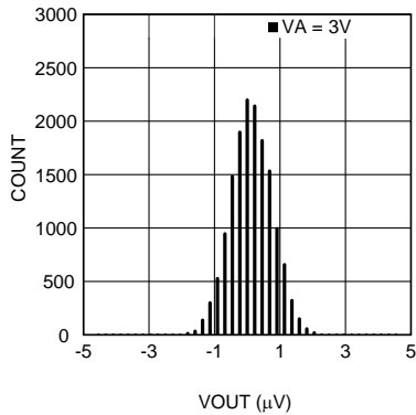
Histogram without Calibration at Gain = 128
