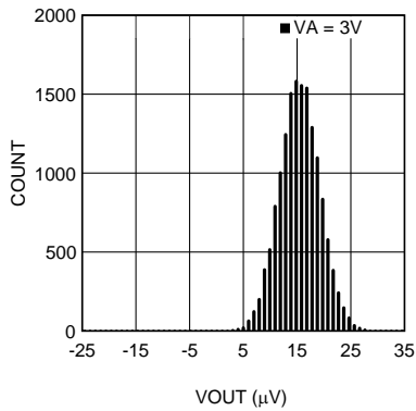
Noise Measurement without Calibration at Gain = 128
