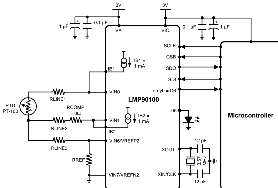
Figure 38. Topology #1: 3-wire RTD Using 2 Current Sources
