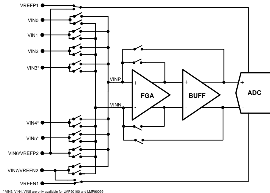
Figure 3. Simplified VIN Circuitry
