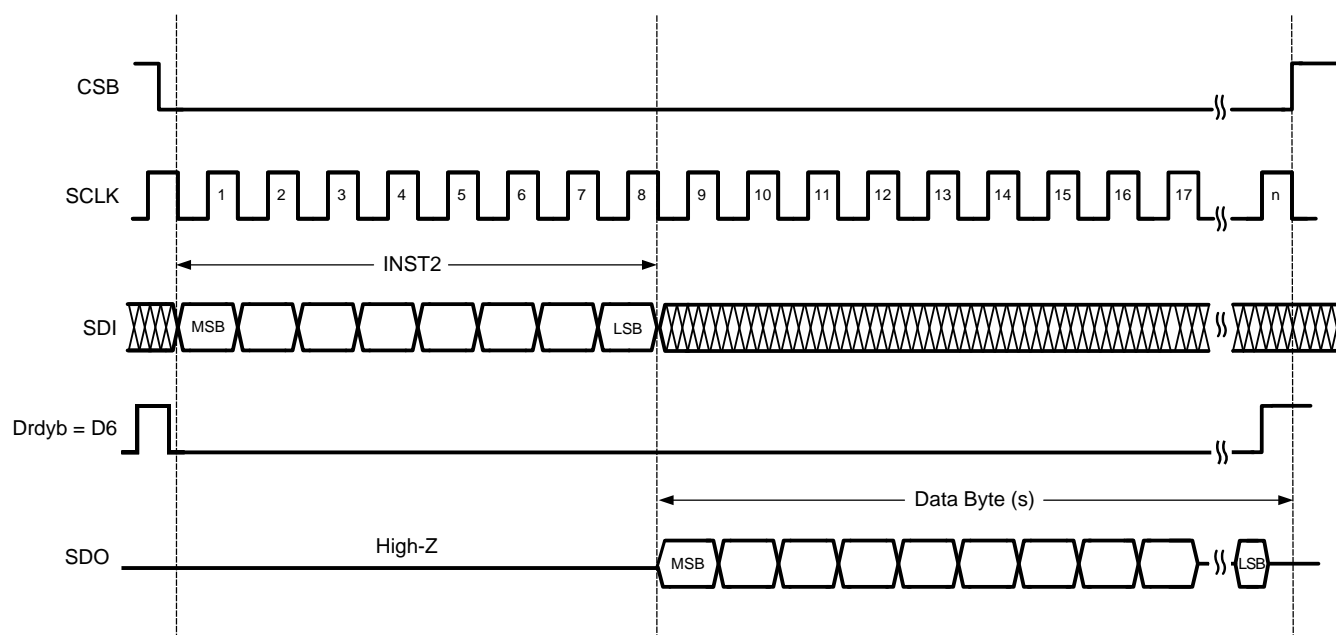
Figure 27. Timing Protocol for DrdybCase3
