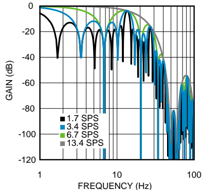
Digital Filter Frequency Response
