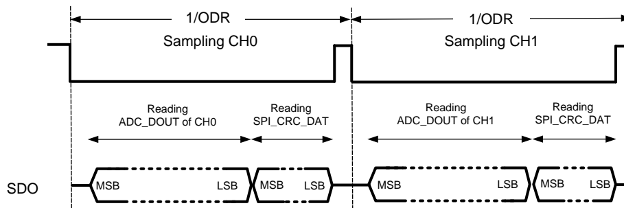
Figure 28. Timing Protocol for Reading SPI_CRC_DAT
