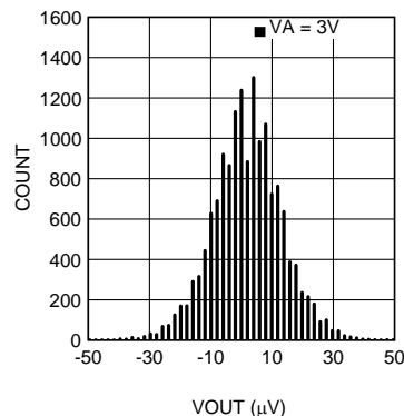
Noise Measurement with Calibration at Gain = 8
