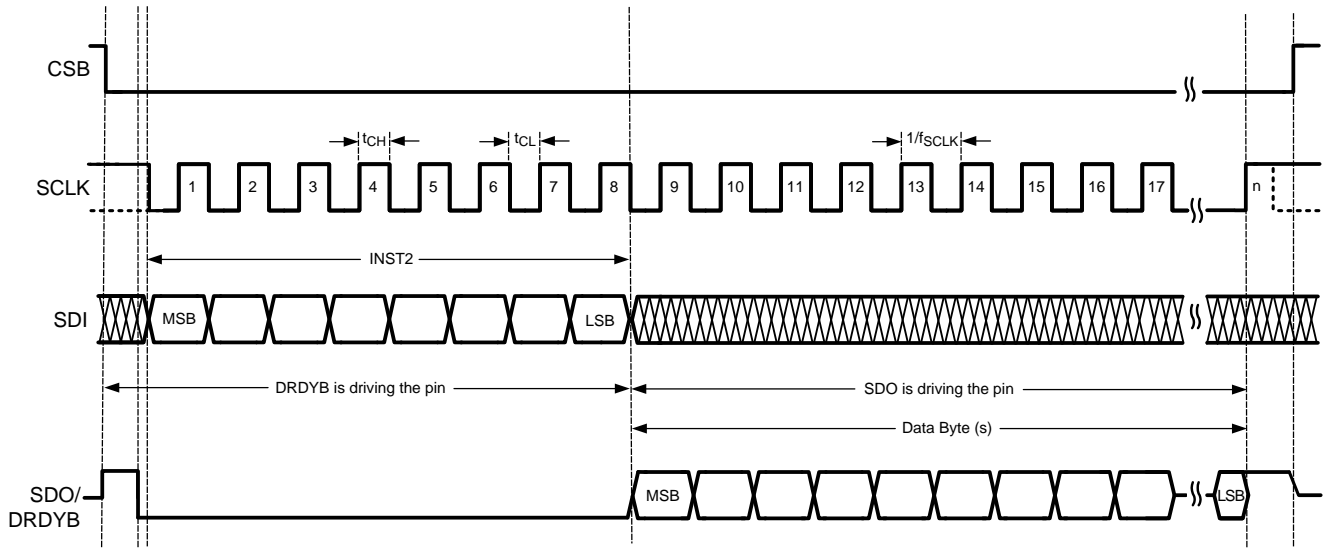
Figure 24. Timing Protocol for DrdybCase1
