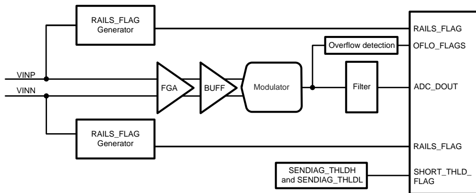
Figure 18. Sensor Diagnostic Flags Diagram
