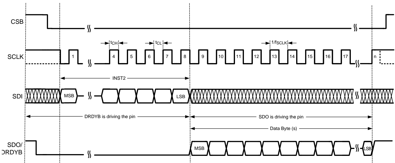
Figure 25. Timing Protocol for DrdybCase2
