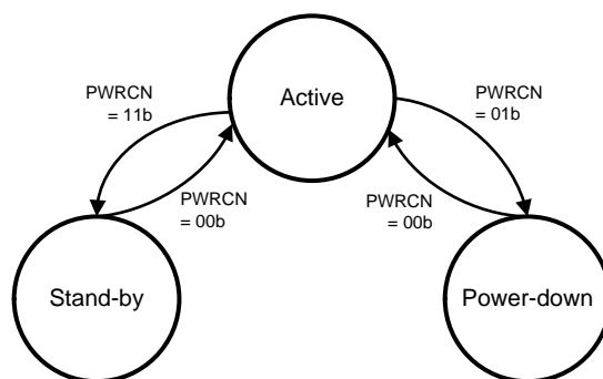
Figure 30. Active, Power-Down, Stand-by State Diagram
