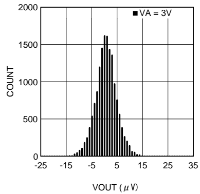
Noise Measurement without Calibration at Gain = 128
