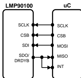
Figure 23. DrdybCase1 Connection Diagram
