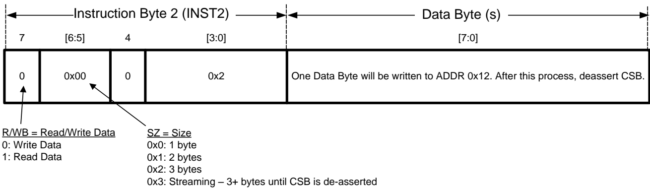
Figure 33. Register-Write Example 2
