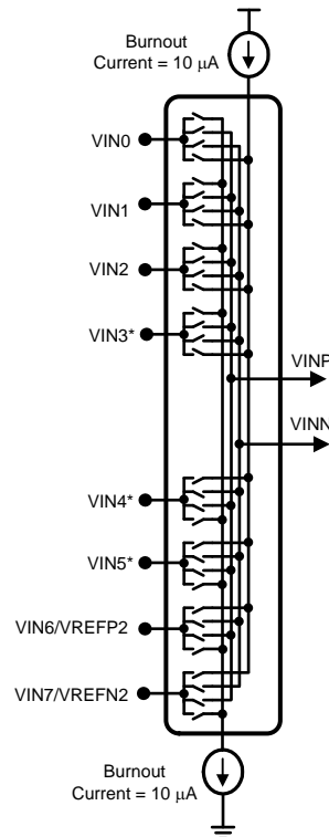
Figure 16. Burnout Currents
