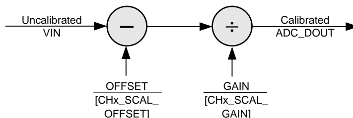
Figure 14. System Calibration Data-Flow Diagram
