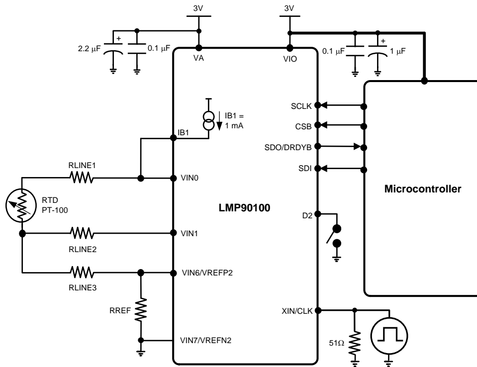
Figure 39. Topology #2: 3-wire RTD Using 1 Current Source
