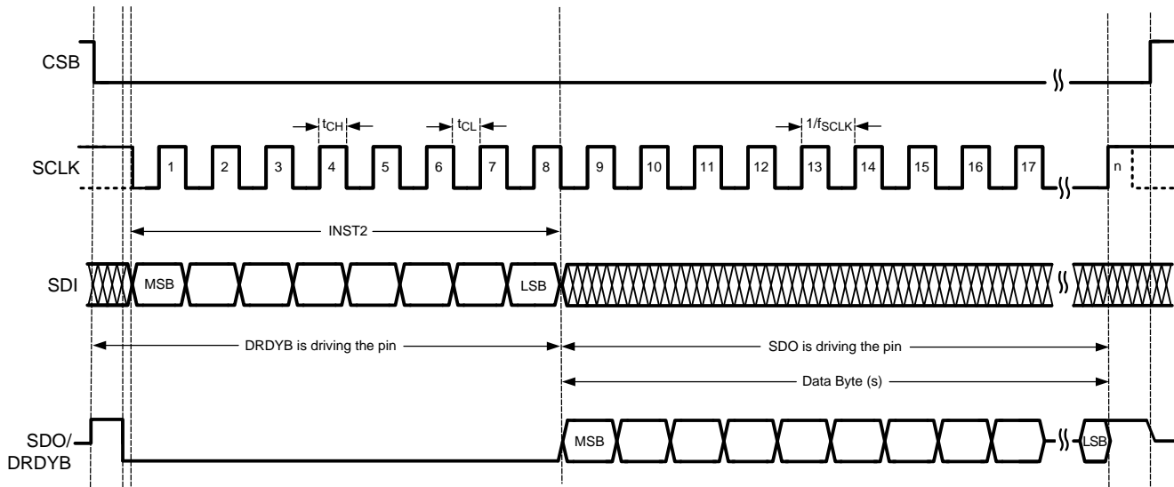
Figure 2. Timing Diagram
