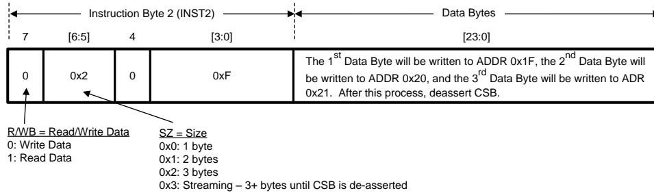
Figure 32. Register-Write Example 1
