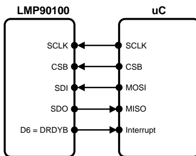
Figure 26. DrdybCase3 Connection Diagram
