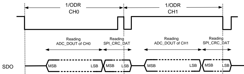
Figure 29. Timing Protocol for Reading SPI_CRC_DAT beyond normal DRDYB deassertion at every 1/ODR seconds
