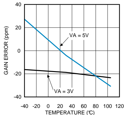
Gain Error vs. Temperature with Calibration at Gain = 8
