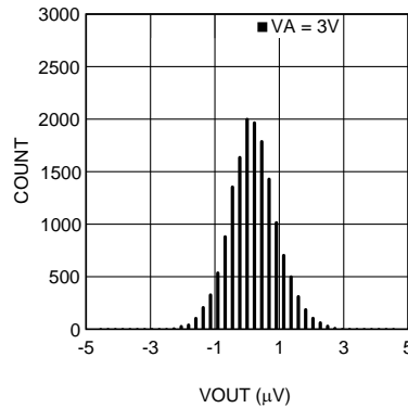
Histogram with Calibration at Gain = 128
