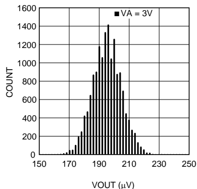
Noise Measurement without Calibration at Gain = 8
