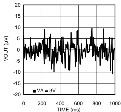
Noise Measurement with Calibration at Gain = 8
