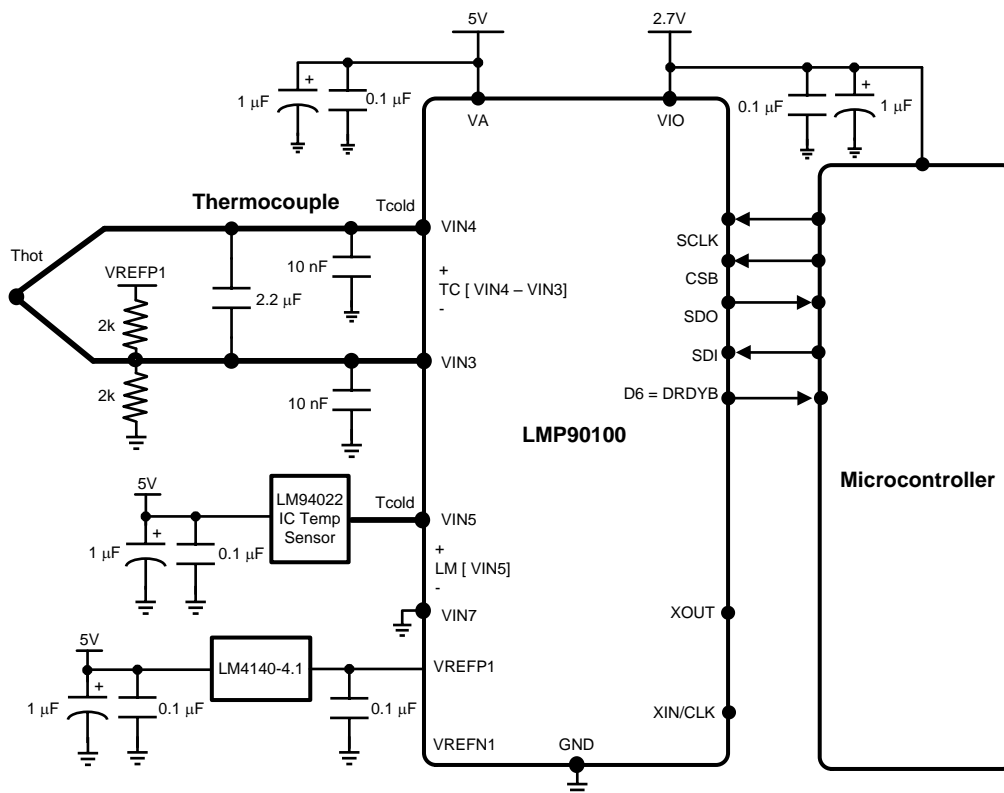
Figure 40. Thermocouple with CJC
