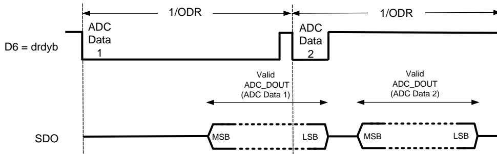
Figure 22. DRDYB Behavior for an Incomplete ADC_DOUT Reading
